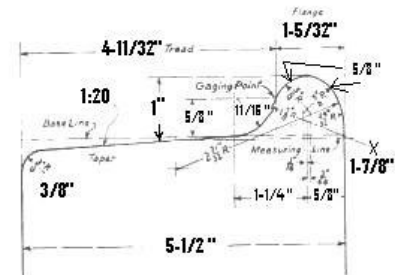
Tread and Flange for Wrought Steel Wheels
